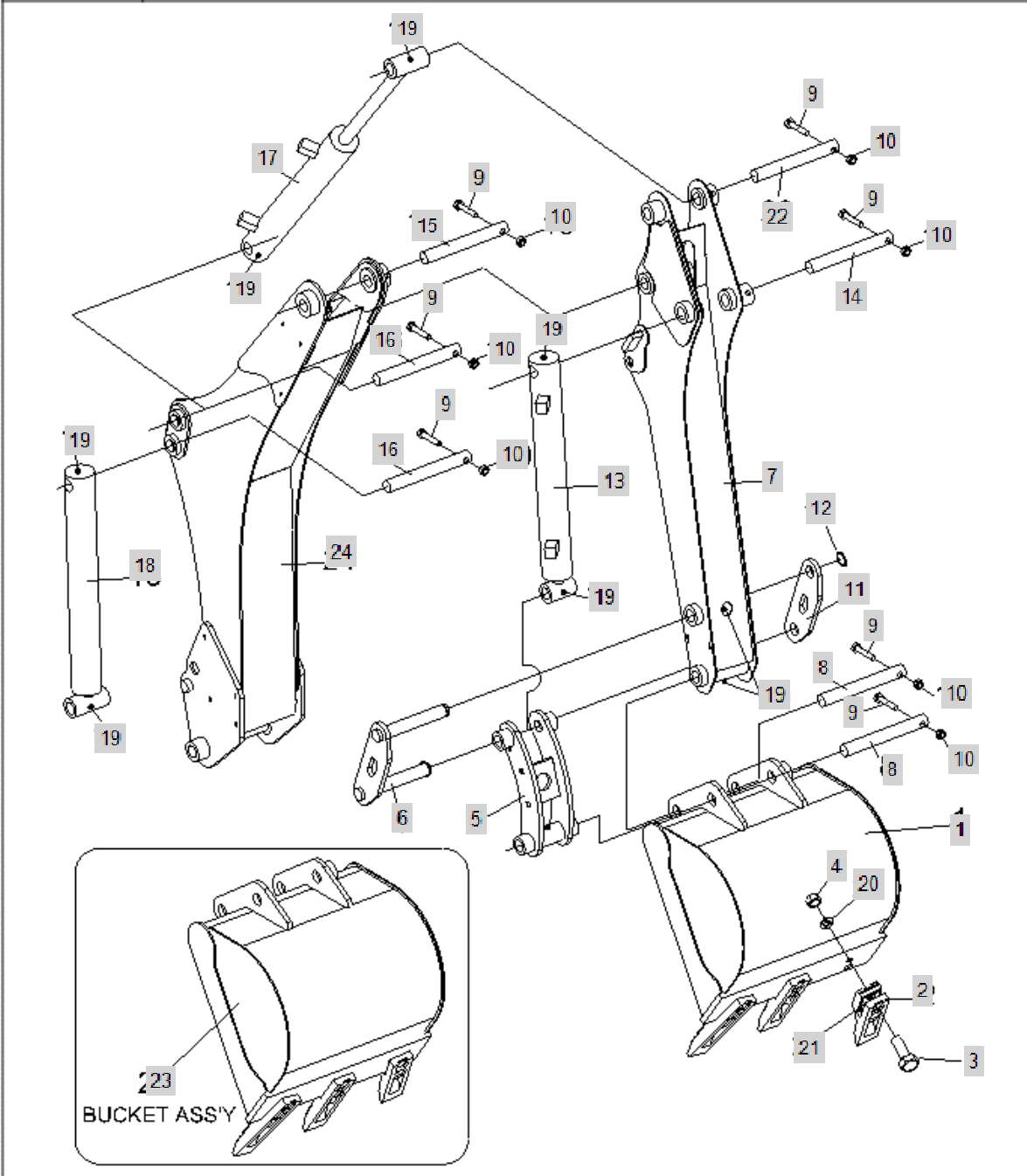
FIG.201 BUCKET, DIPPER STICK, BOOM
